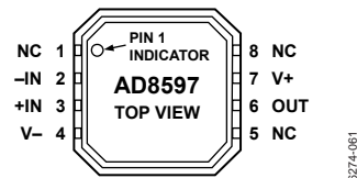
Figure 1. AD8597 8-Lead SOIC (R-8)
